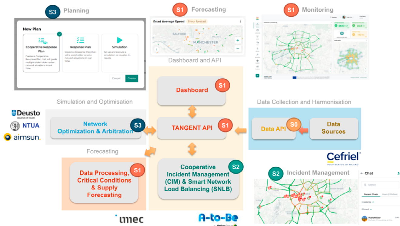
Figure 4 - The TANGENT Tool Architecture (Source: A-to-Be).
