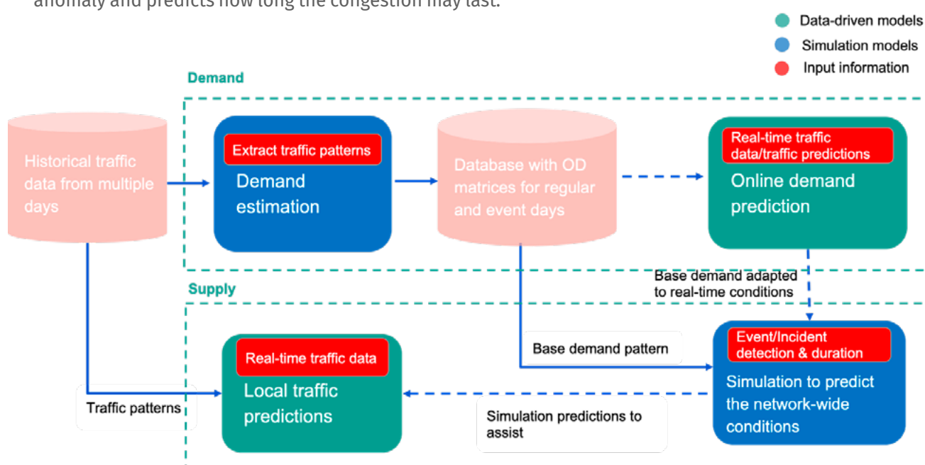
Figure 8 - Real-time traffic management framework (Source: Aimsun).
