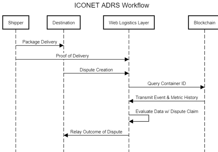
Figure 1 - ADRS Workflow
