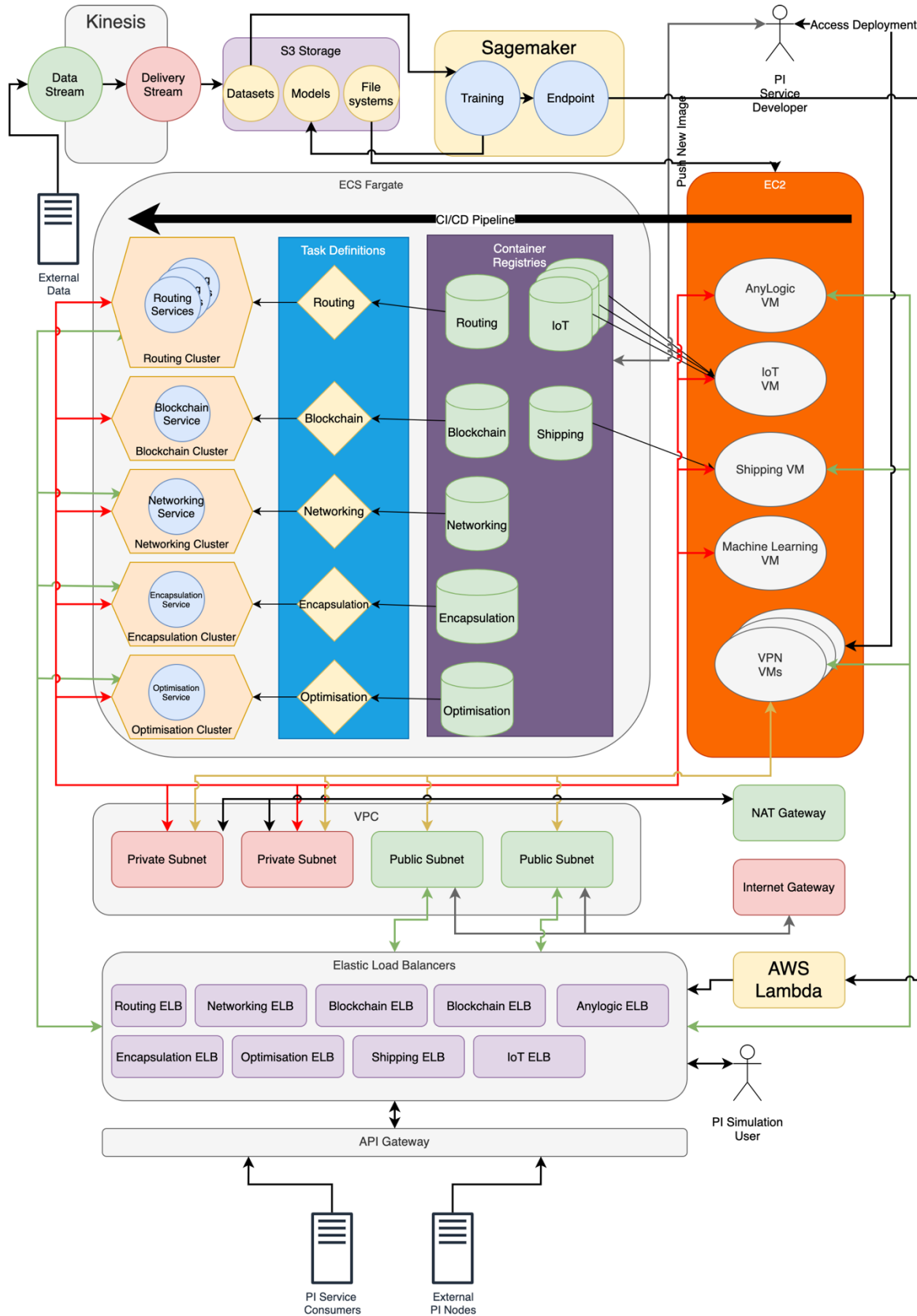
Figure 23 - PoC Blueprint
