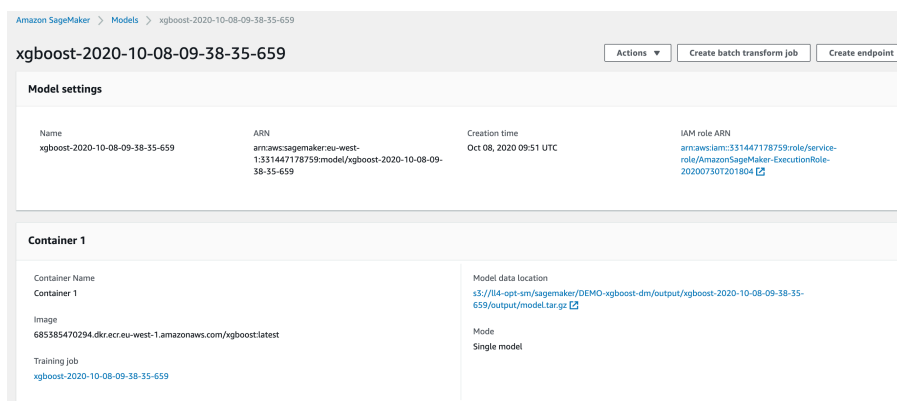
Figure 18 - Saved Model
