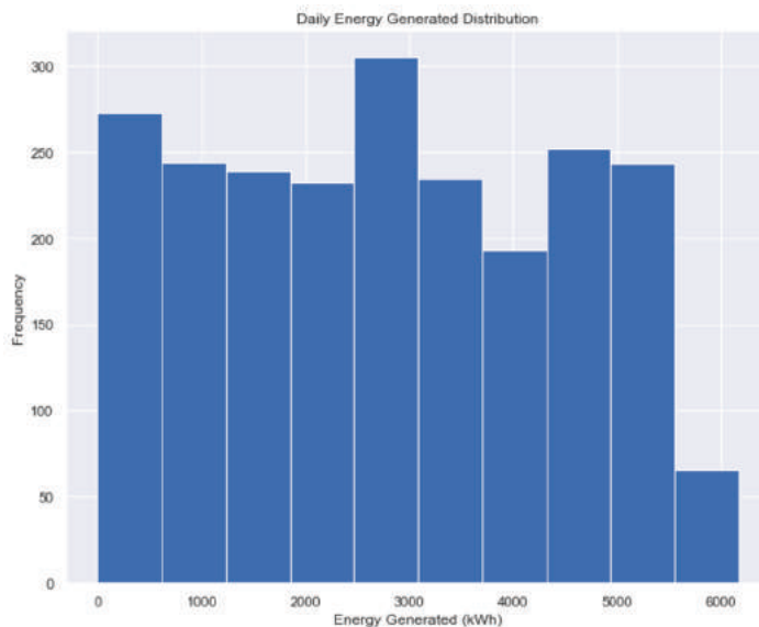
Figure 66. Photovoltaic daily production distribution
