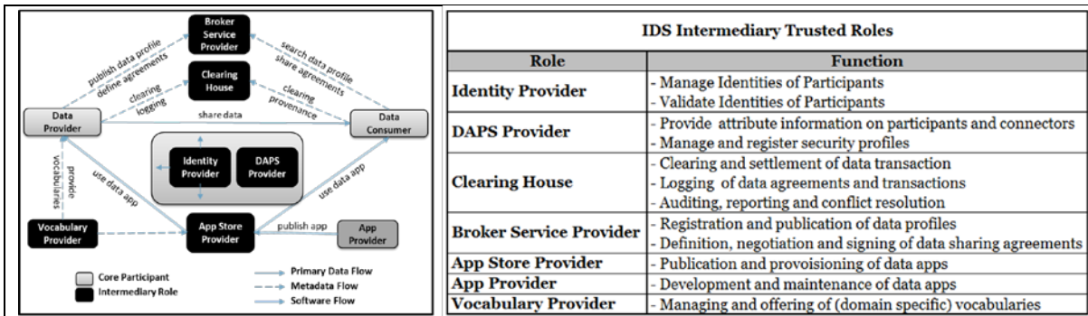
Figure 3: Roles in the IDS Reference Architecture (l) (Otto et al. 2019), together with a Functional Description for the Intermediary Roles (r) (Dalmolen et al. 2018).
