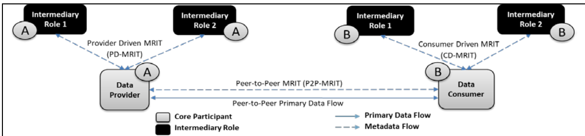
Figure 5: Runtime Environment for Metadata Flow Control based on Data Sharing Connectors.
