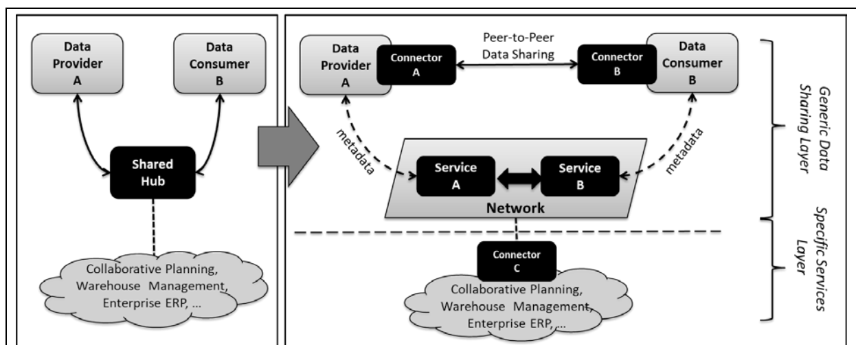
Figure 2: Transition from a Hub-Model Approach (l) to an Open Network-Model Approach (r) for Data Sharing (Liezenberg et al. 2018).
