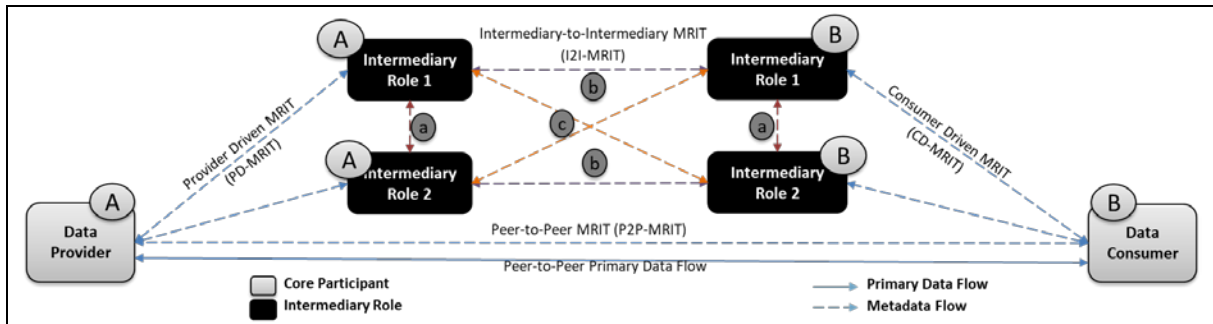
Figure 4: Metadata Interaction Patterns within the Generic Data Sharing Layer in a Distributed Open Network-Model Approach.
